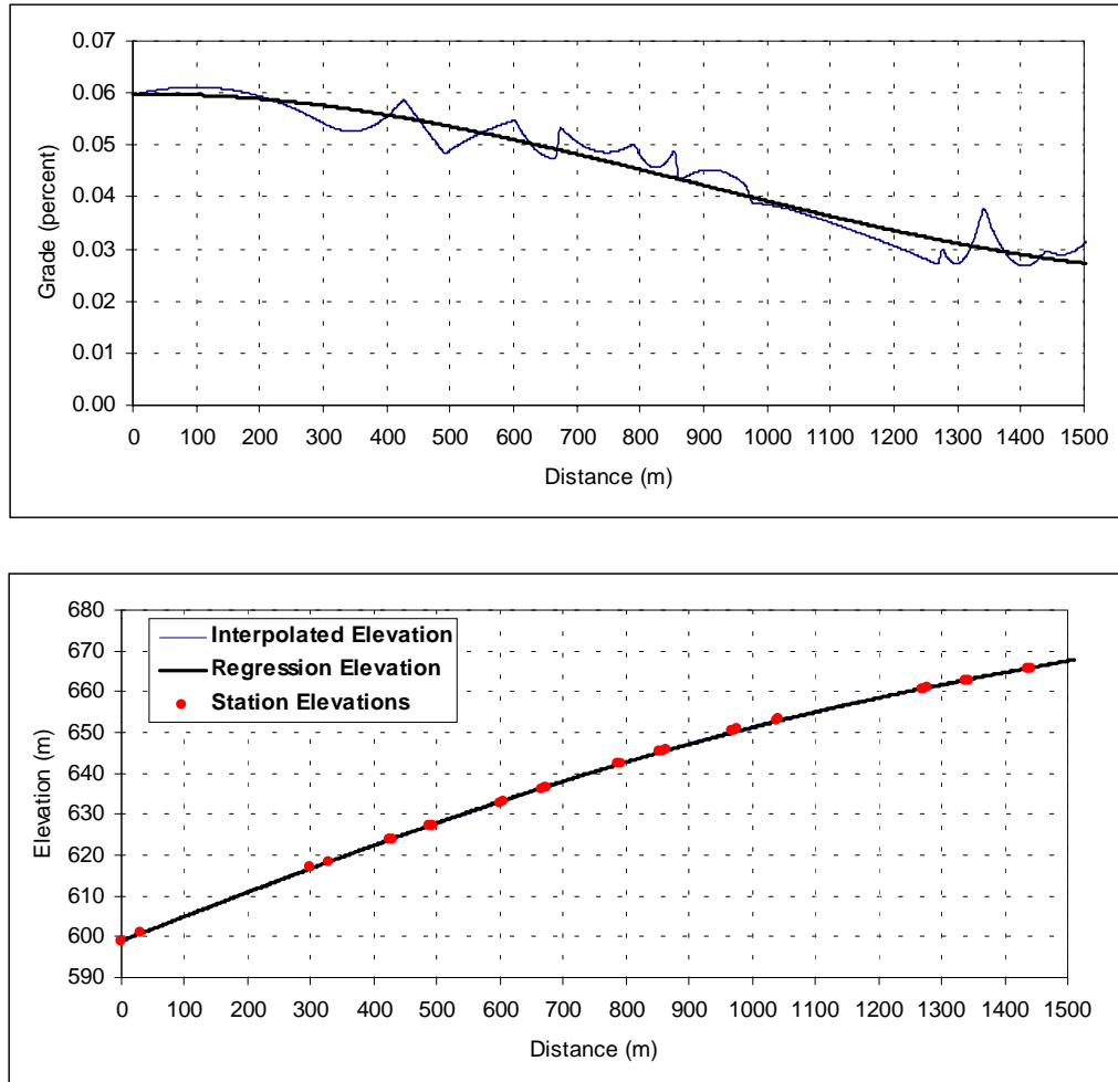
Figure 3. Smart Road test section longitudinal profile
