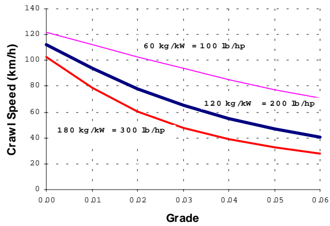
Figure 6. Variation in equilibrium speed as a function of roadway grade for NTC-350 engine
