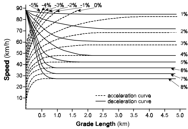
Figure 2. Truck performance curves for an average truck (120 kg/kW or 200 lb/hp) [HCM, 1998]
