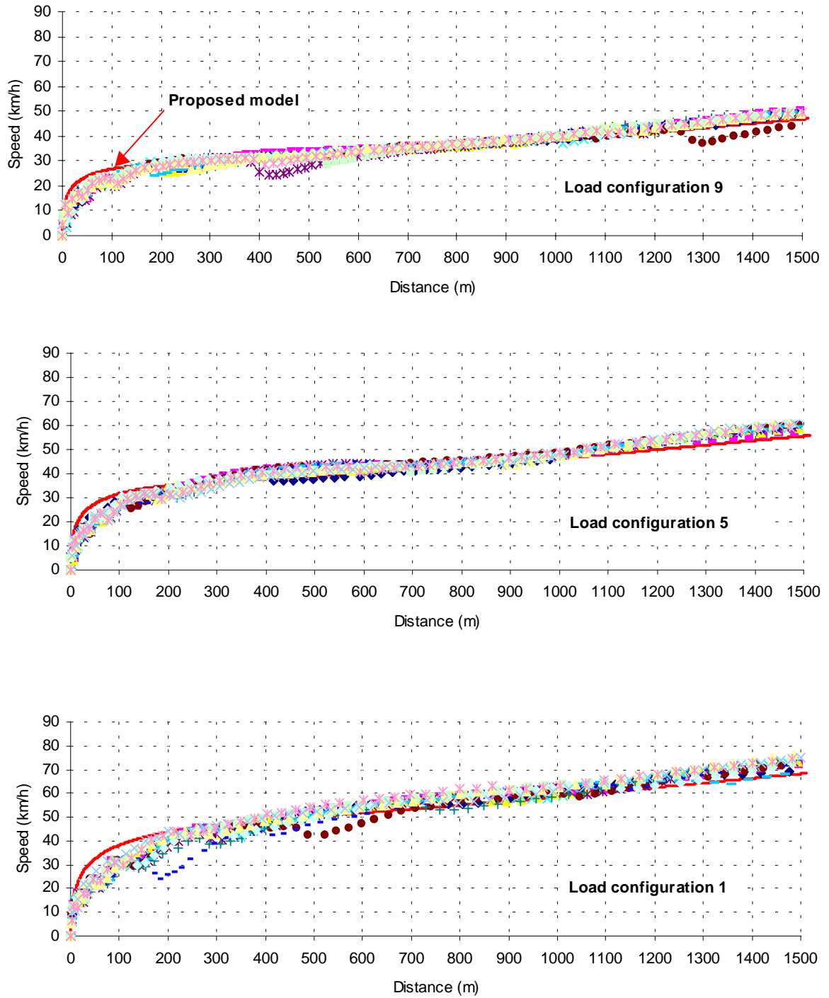
Figure 4. Predicted and observed speed profile for selected load configurations
