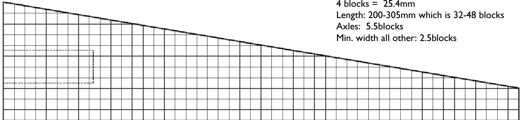
SIDE VIEW
