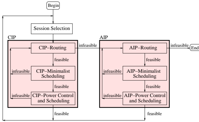
Fig. 1. Flow chart of our algorithm.
