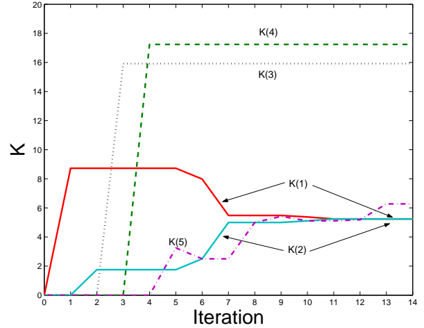
Fig. 3. Iterations for scaling factor of each session during the simulation.
