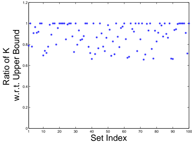
Fig. 4. Ratio of K w.r.t. upper bound for 100 data sets.
