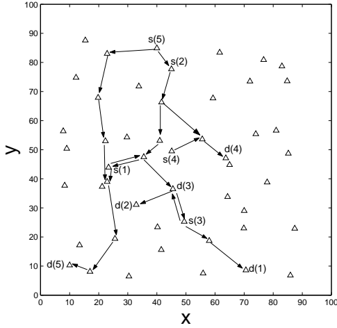
Fig. 2. 50-node CR network with 5 active sessions.
